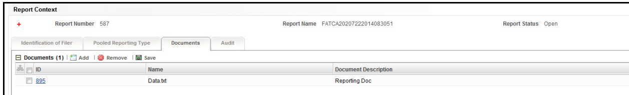
Figure 26. Documents Tab
