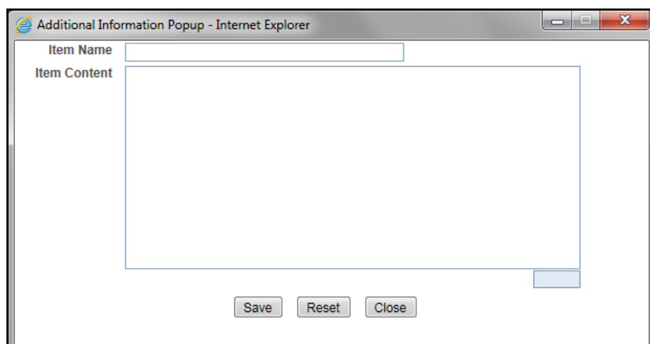
Figure 23. Additional Information
